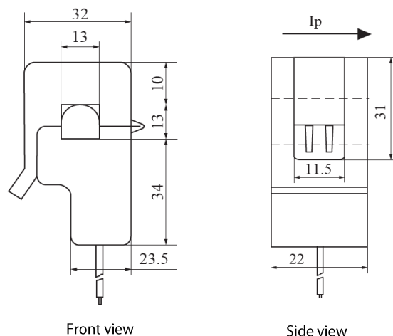
Enclosure dimensions 100A Current Transformer (dimensions in mm)
